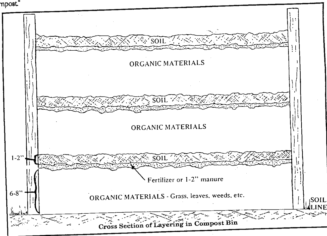
Figure 7. A cross section of a properly constructed compost pile.
