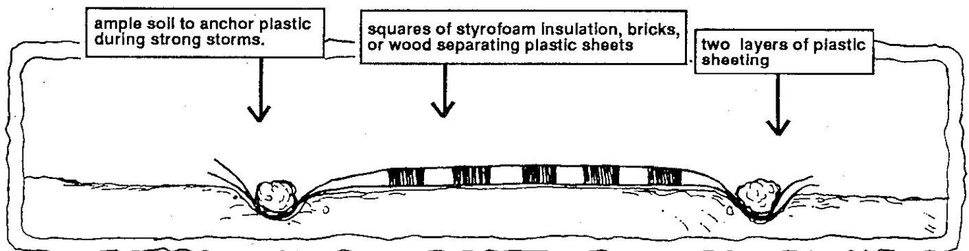
Figure 2. Soil solarization procedure.
